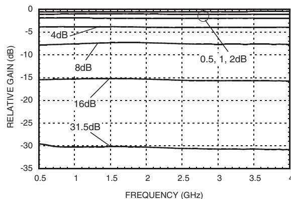
Input Attenuator Relative Attenuation (Major States)
