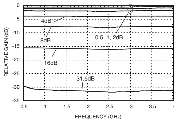
Output Attenuator Relative Attenuation (Major Steps)
