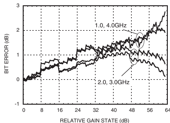
Input Attenuator Bit Error vs. Attenuation State (Major Frequencies)
