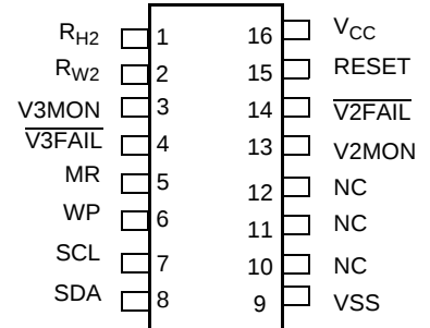
X40235 16 Pin SOIC
