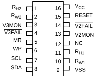
X40239 16 Pin SOIC
