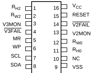
X40237 16 Pin SOIC
