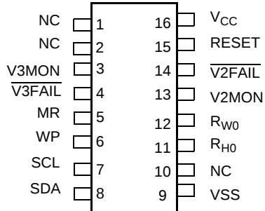
X40231 16 Pin SOIC
