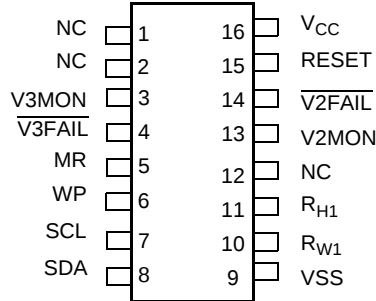
X40233 16 Pin SOIC
