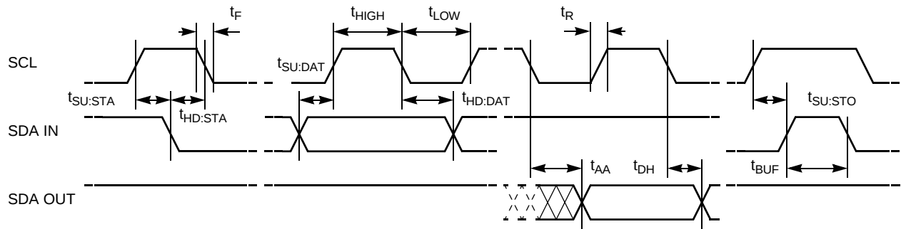
Figure 27. Bus Timing
