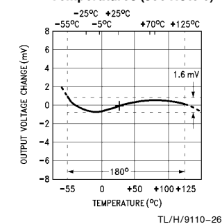
LM169 Temperature Coefficient Specified Temperatures (see Note 6)
