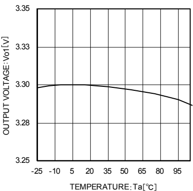
Fig. 22 Output Voltage vs Temperature (3.3 V output)
