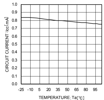
Fig. 24 Circuit Current vs Temperature
