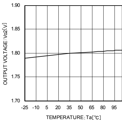
Fig. 23 Output Voltage vs Temperature (Variable output: 1.8 V)
