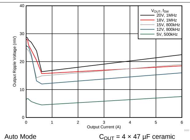
图 26. Voltage Ripple vs Output Current
