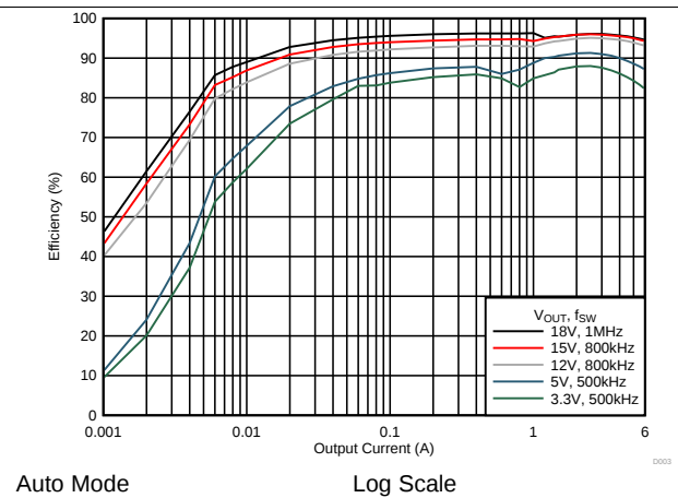
图 14. Efficiency vs Output Current
