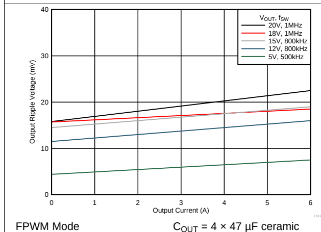
图 25. Voltage Ripple vs Output Current
