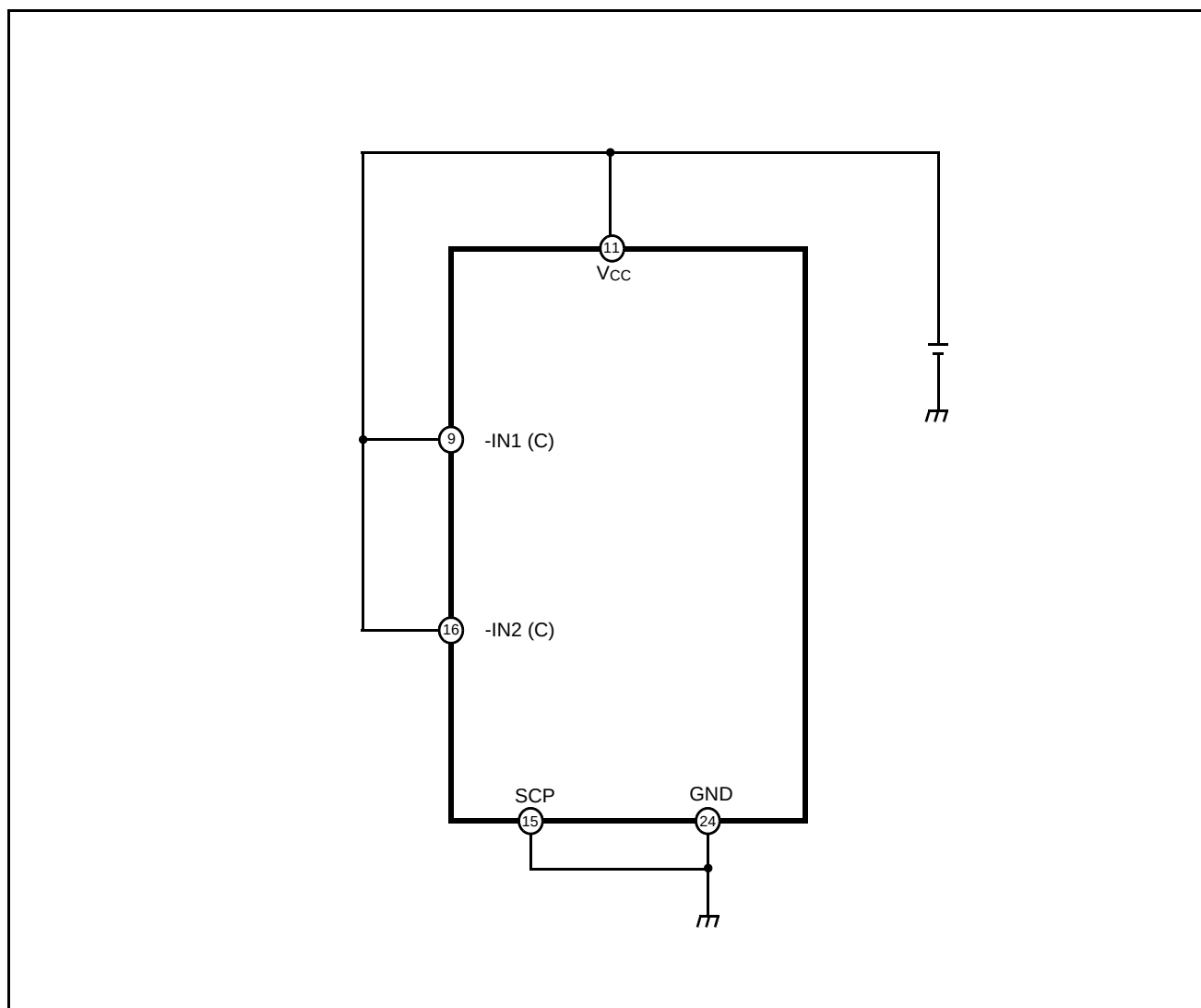
Fig. 6 Processing without using SCP Pin
