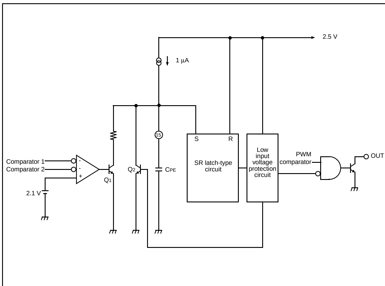
Fig. 5 Latch-Type Short-Circuit Protection Circuit
