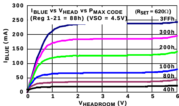
FIGURE 3. I_{\text{BLUE}} WRITE CURRENT vs V_{\text{HEADROOM}} vs P_{\text{MAX}}
