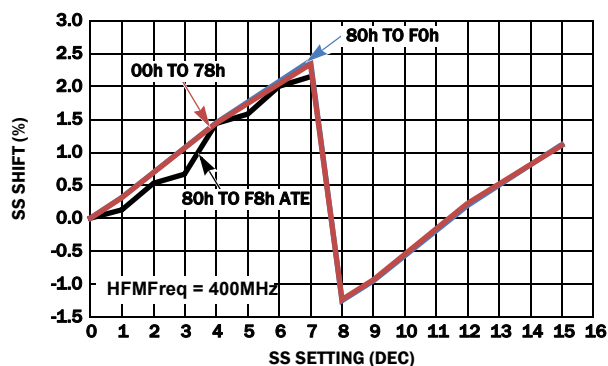
FIGURE 8. I_{\text{BLUE}} SS SHIFT vs SS SETTING @ 400MHz
