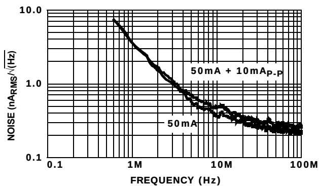
FIGURE 9. I_{BLUE} NOISE vs FREQUENCY
