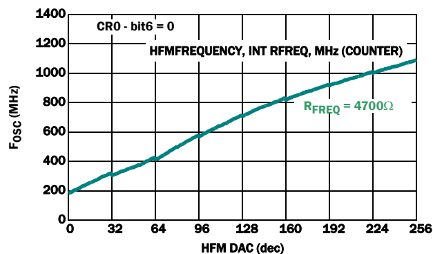
FIGURE 6. HFM CONTROL; V_{\text{SO}} = 5.0\text{V}
