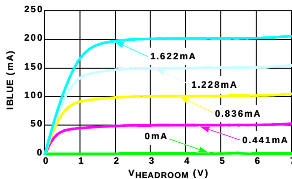
FIGURE 4. I_{\text{BLUE}} READ vs V_{\text{HEADROOM}} vs I_{\text{AP}} (REG 1-21 = 88h) ( V_{\text{SO}} = 5.0\text{V} ), ( R_{\text{SET}} = 620\Omega )
