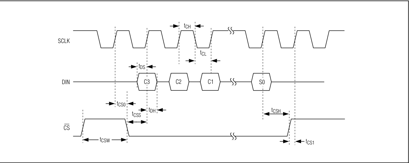
Figure 1. Timing Diagram
