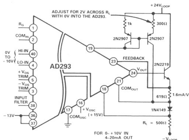
Figure 15. Isolated Current Loop Interface
