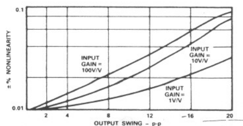
Figure 11. Typical AD293/AD294 - Gain Nonlinearity vs. Output Swing
