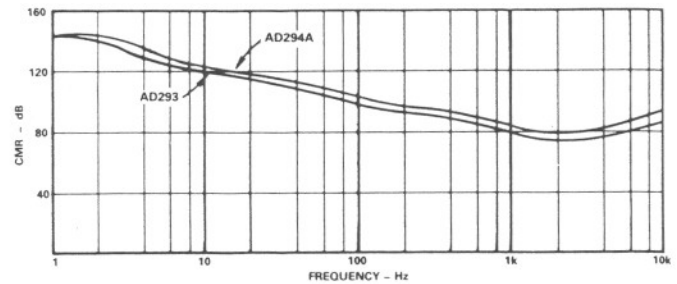
Figure 6. Typical AD293/AD294 - CMR vs. Frequency
