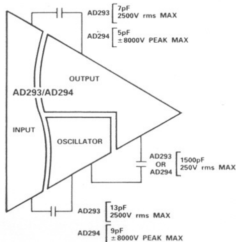
Figure 3. Interelectrode Capacitance and Terminal Ratings
