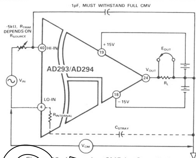
Figure 13. Improving CMR by Cancellation
