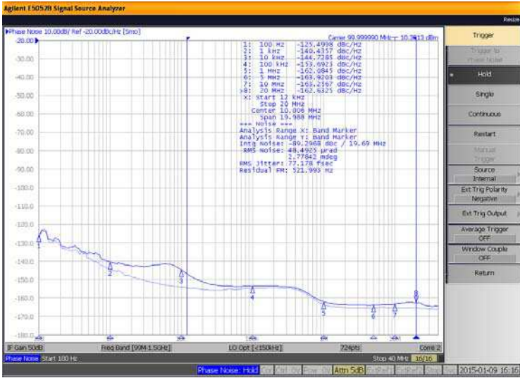
Figure 2. 551S Output Phase Noise 77fs (12kHz to 20MHz)
