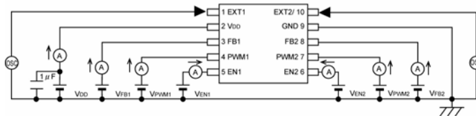
Circuit 3
