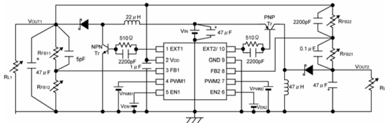
Circuit 2
