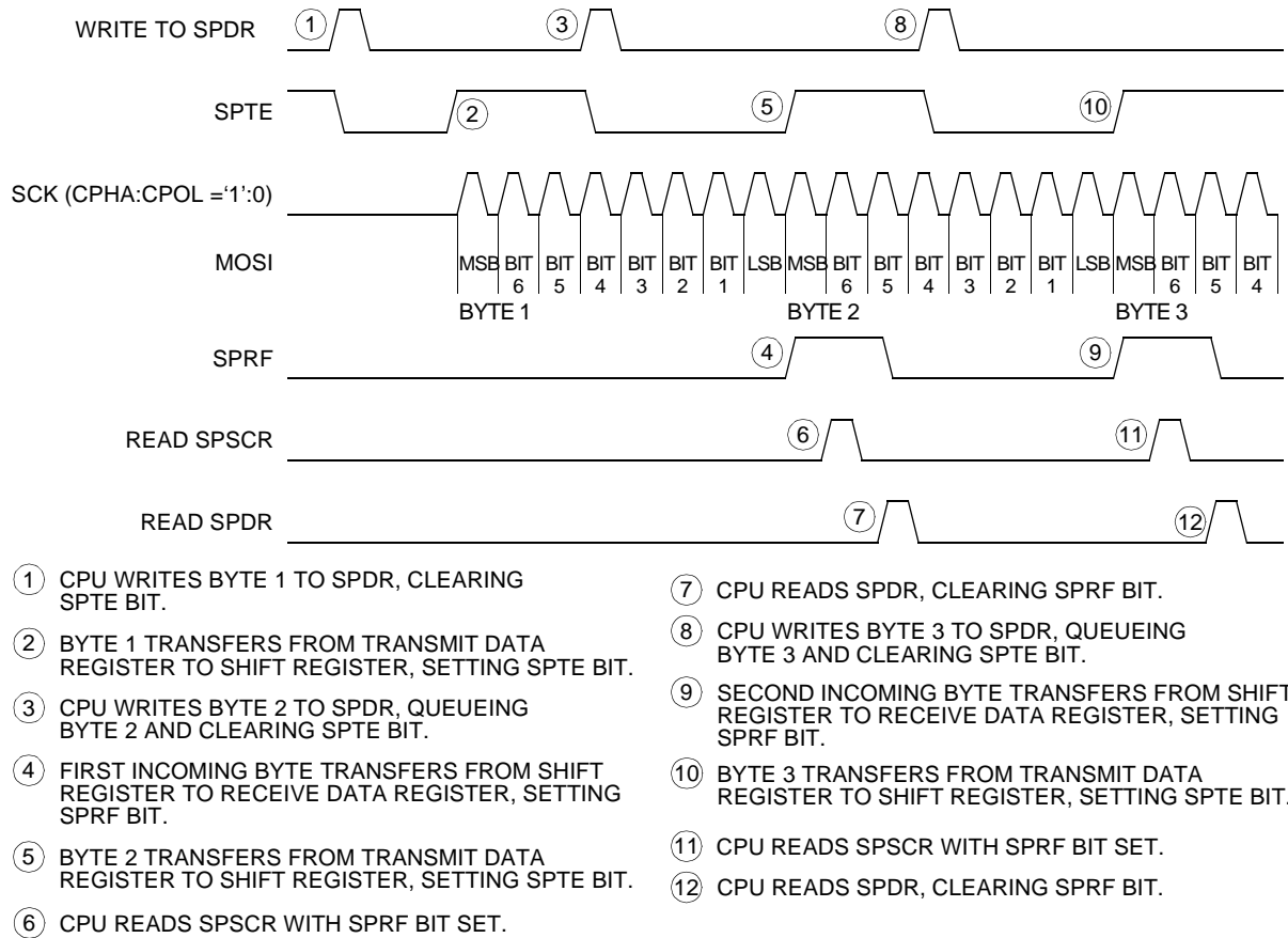
Figure 17-10. SPf/SPTe CPU Interrupt Timing
