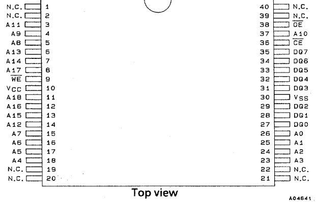
TSOP40 Reversed
