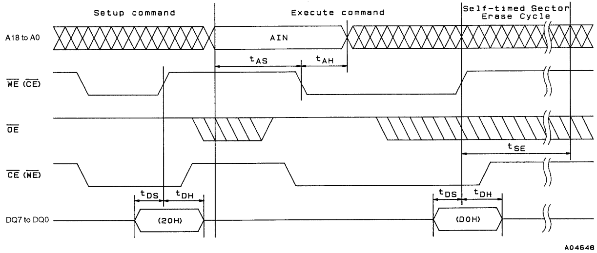
Figure 6 Sector Erase
