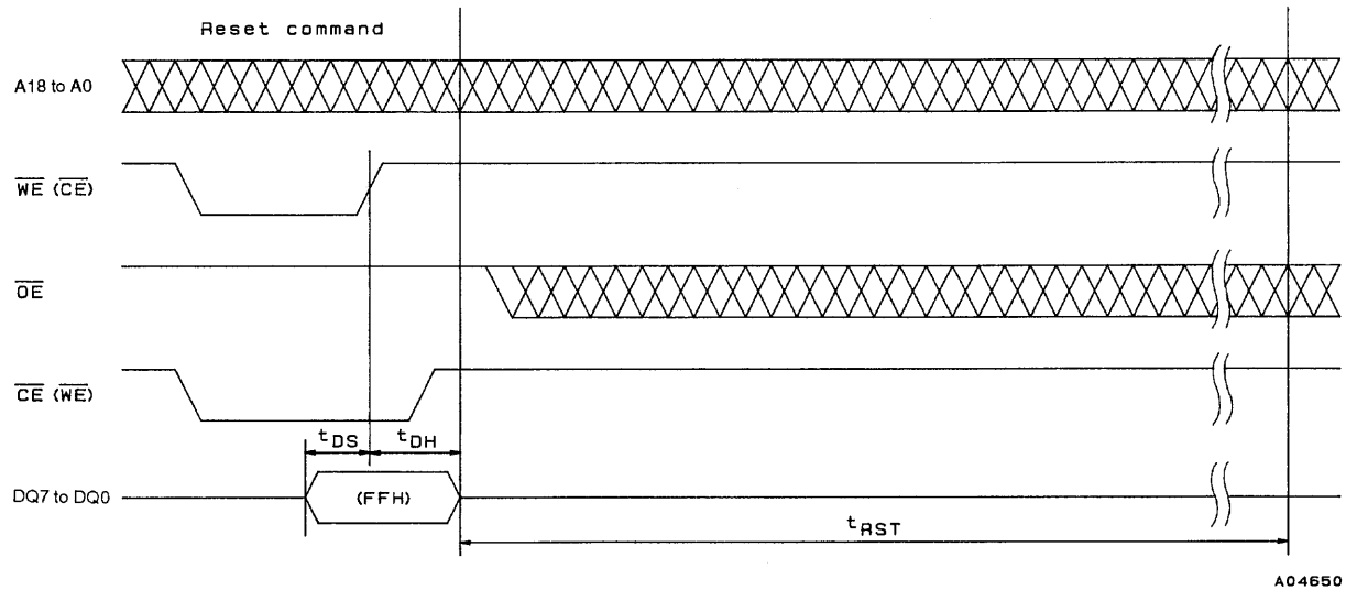
Figure 8 Reset
