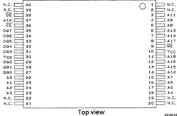
TSOP40 Standard
