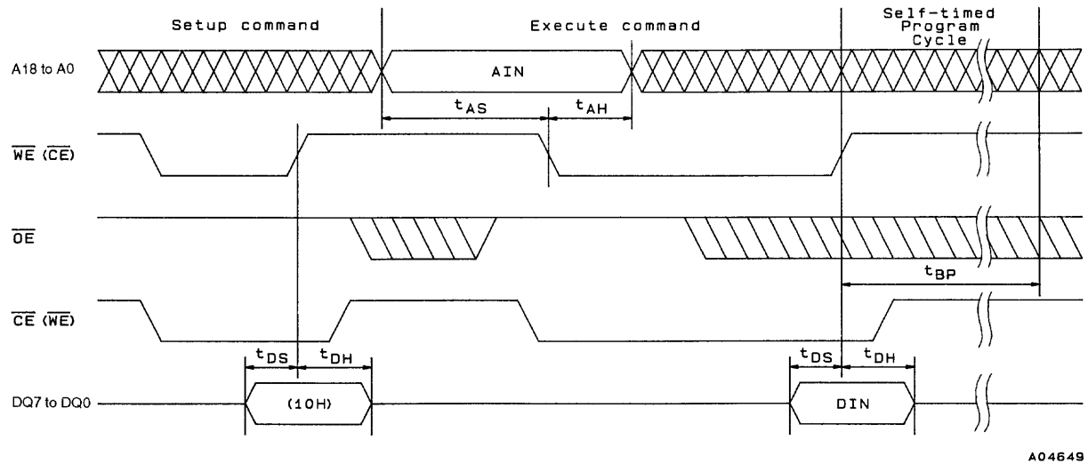
Figure 7 Byte Programming
