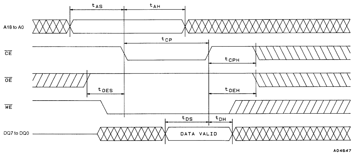
Figure 5 \overline{\text{CE}} Control Write Cycle
