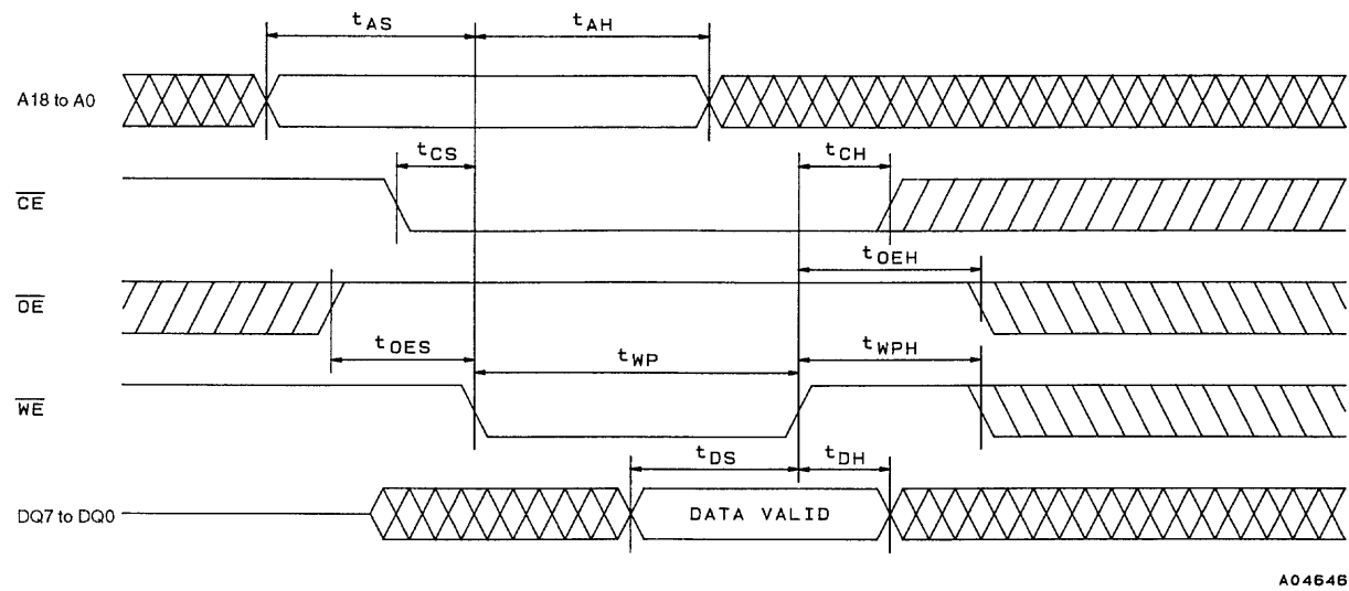
Figure 4 \overline{\text{WE}} Control Write Cycle
