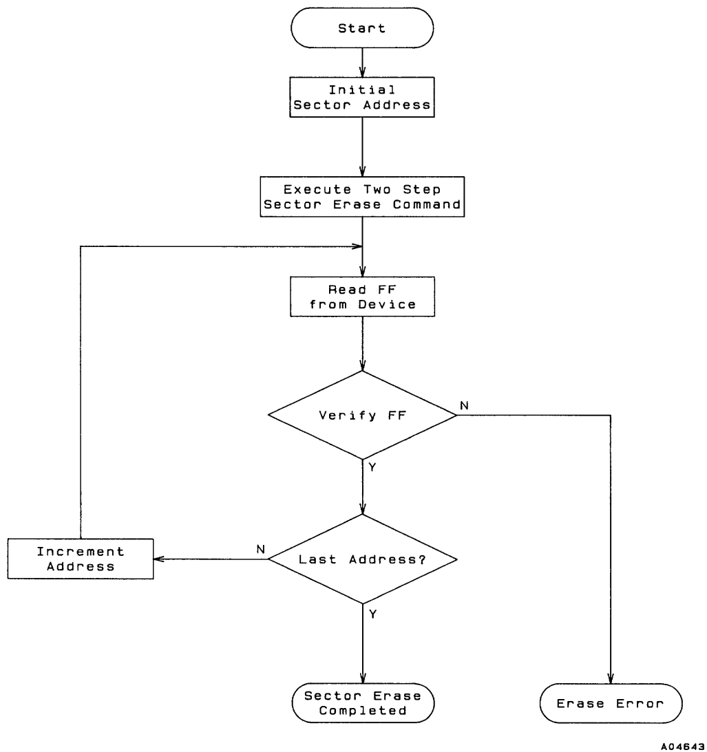
Figure 1 Sector Erase Flowchart
