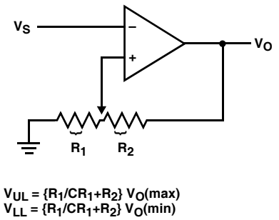
COMPARATOR WITH HYSTERITISIS
