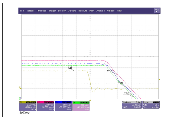
FIGURE 1-17: Typical \overline{\text{LATCHC}} to \text{HV}_{\text{OUT}} Propagation Delay.
