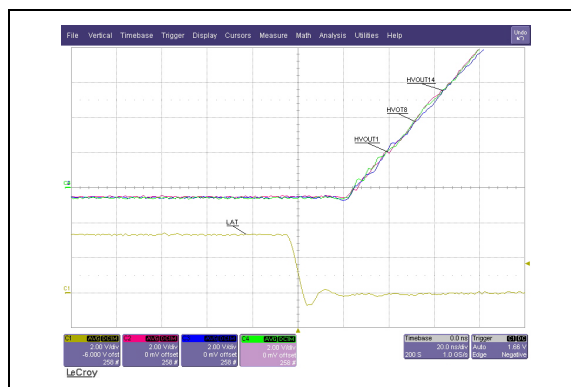
FIGURE 1-20: Typical \overline{\text{LATCHD}} to \text{HV}_{\text{OUT}} Propagation Delay.
