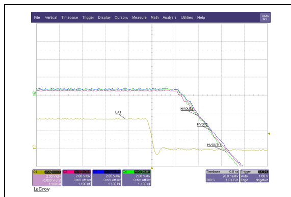
FIGURE 1-19: Typical \overline{\text{LATCHB}} to \text{HV}_{\text{OUT}} Propagation Delay.
