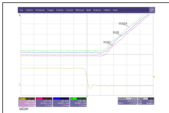
FIGURE 1-16: Typical \overline{\text{LATCHA}} to \text{HV}_{\text{OUT}} Propagation Delay.
