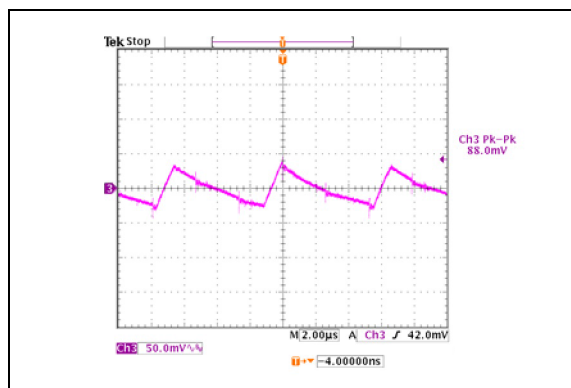
FIGURE 1-21: Typical Charge Pump Output Noise Ripple.
