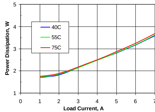
Figure 5. Power dissipation vs. load current and ambient temperature for SSQE48T07050 converter mounted vertically with V_{in} = 48\text{ V} and air flowing from pin 1 to pin 3 at a rate of 200 LFM (1.0 m/s).
