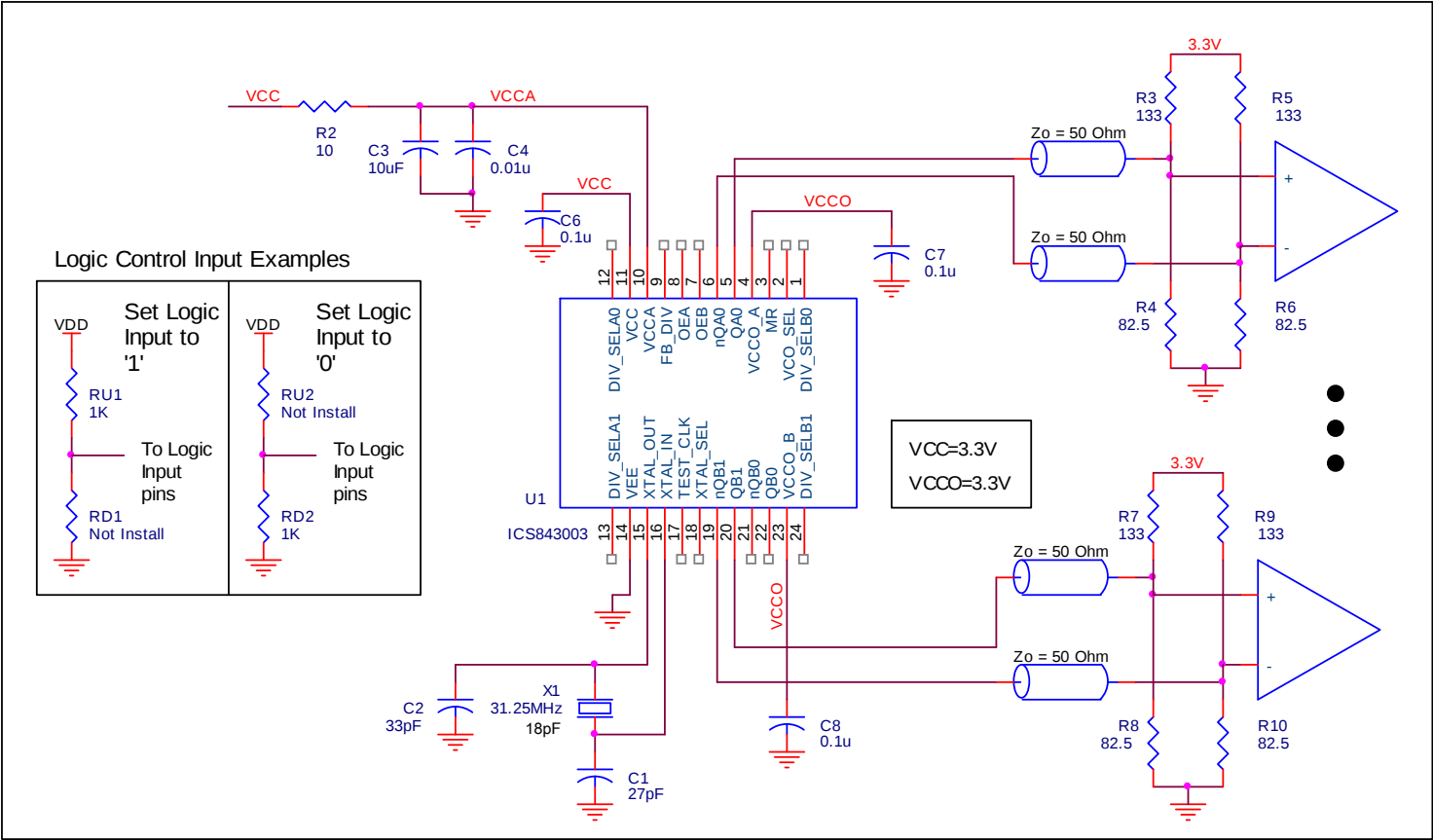
Figure 6A. 843003 Schematic Example
