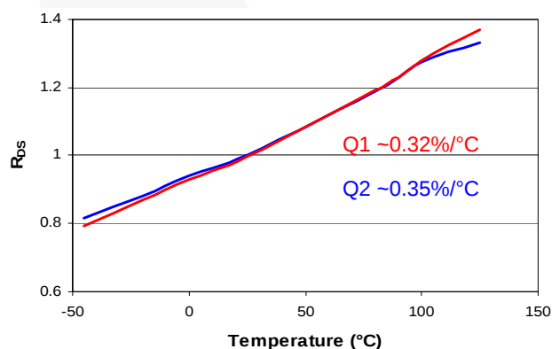
Figure 8. R_{DS} vs. Temperature, Normalized ( V_{CC}=V_{GS}=5 V), Figure 1
