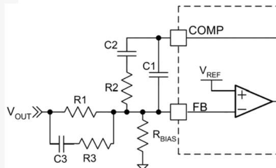
Figure 34. Compensation Network
