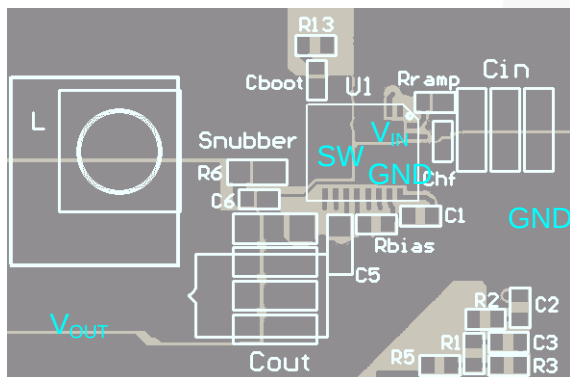
Figure 35. Recommended PCB Layout
