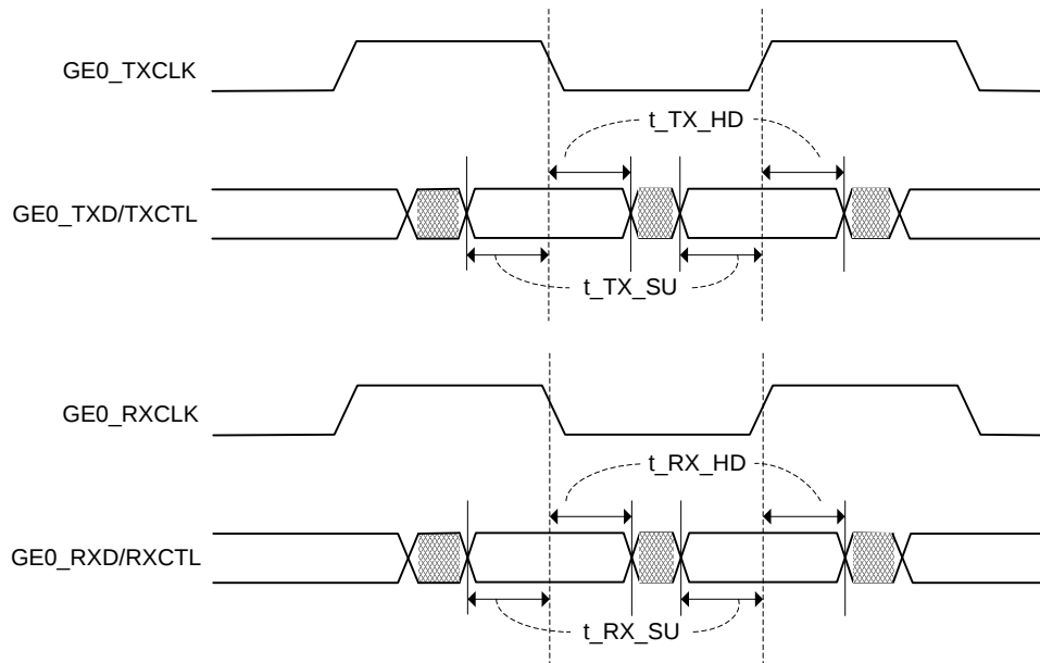
Figure 3-5 RGMII Interface
