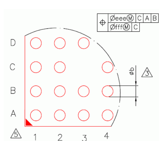
Figure 3-16 TFBGA "B" Expanded
