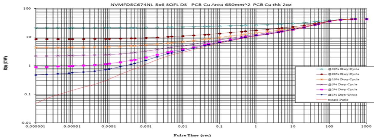
Figure 13. Thermal Characteristics
