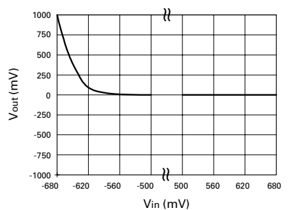
REC DC Transfer Characteristics
