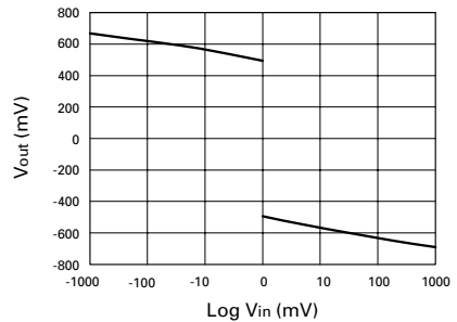
LOG DC Transfer Characteristics
