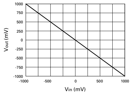
NEG DC Transfer Characteristics
