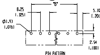
PTH PATTERN
