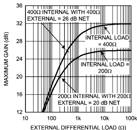
FIGURE 5. Gain vs. External Load
