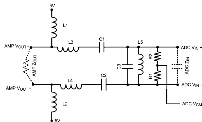
FIGURE 7. Sample Filter
