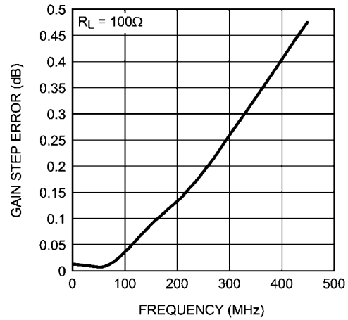
Worst Case Gain Step Error vs. Frequency
