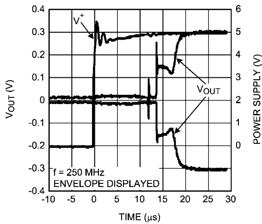
Power On Timing, Minimum Gain
