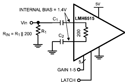
FIGURE 3. Single Ended Input (Note capacitor on grounded input)
