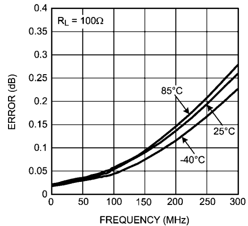
Worst Case Gain Step Error Over Temperature
