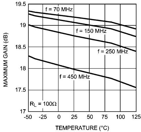
Maximum Gain Over Temperature
