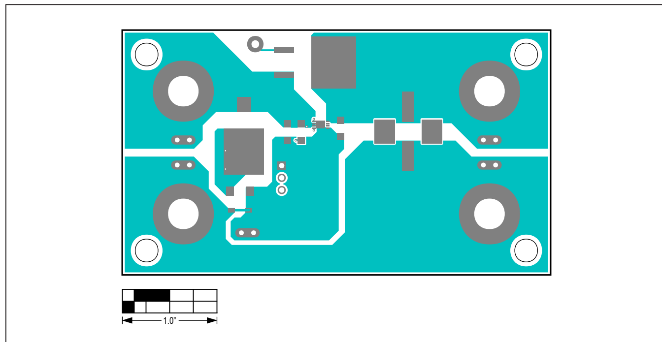
MAX16171 EV Kit PCB Layout—Top View
