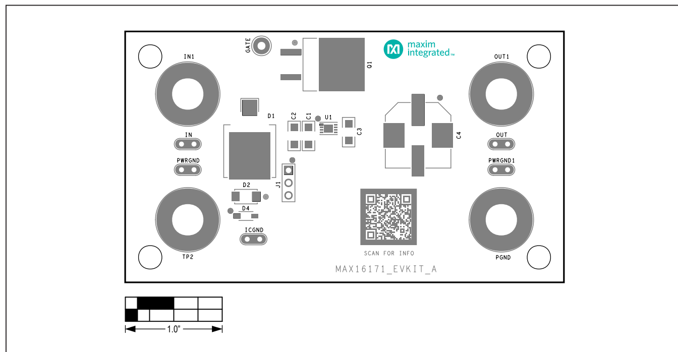
MAX16171 EV Kit PCB Layout—Top Silkscreen
