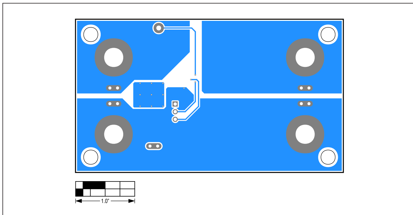
MAX16171 EV Kit PCB Layout—Bottom View
