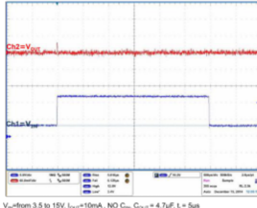
Figure 25. Line transient ( V_{OUT} = 1.2\text{ V} )
