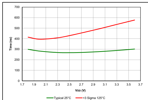
FIGURE 38-70: Comparator Response Time, Rising Edge, PIC16LF18854 Only.
