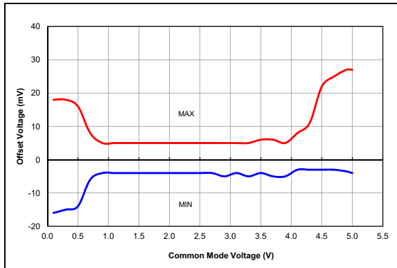
FIGURE 38-55: Comparator Offset, NP Mode ( CxSP = 1 ), V_{DD} = 5.5V , Typical Measured Values from -40^\circ C to 125^\circ C , PIC16F18854 Only.
