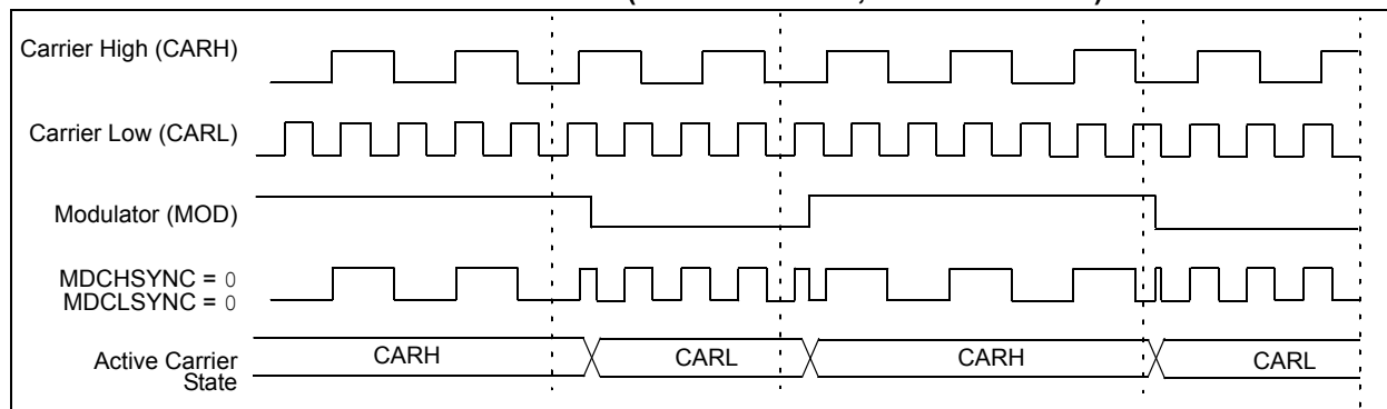
FIGURE 26-3: NO SYNCHRONIZATION (MDSHSYNC = 0, MDCLSYNC = 0)
