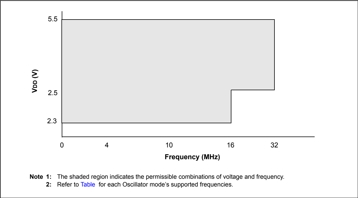
FIGURE 37-2: VOLTAGE FREQUENCY GRAPH, -40^{\circ}\text{C} \leq T_A \leq +125^{\circ}\text{C} , PIC16LF18854 ONLY
