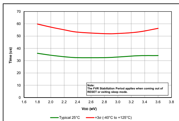
FIGURE 38-72: FVR Stabilization Period, PIC16LF18854 Only.
