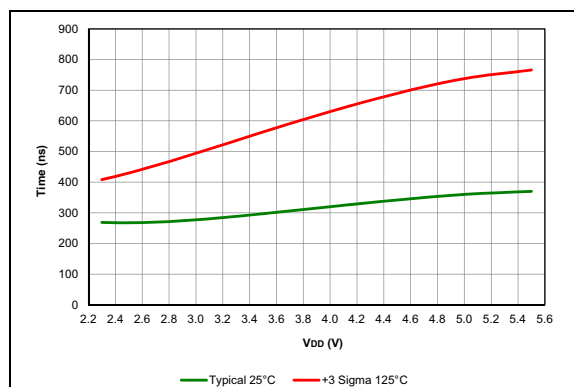
FIGURE 38-71: Comparator Response Time, Rising Edge, PIC16F18854 Only.
