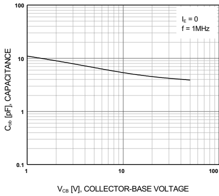
Figure 3. Output Capacitance
