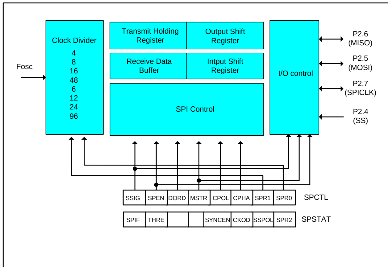
SPI block diagram
