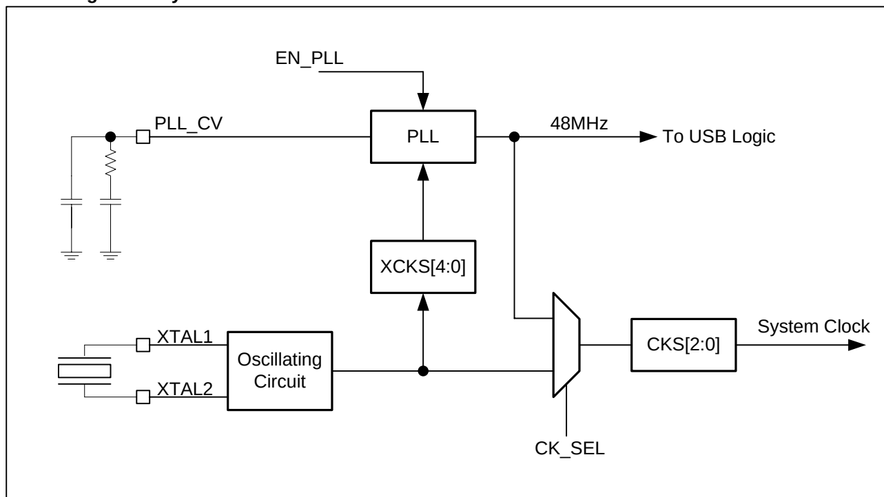
Block Diagram of System Clock
