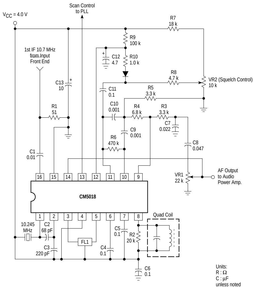
Figure 9. Simplified Application
