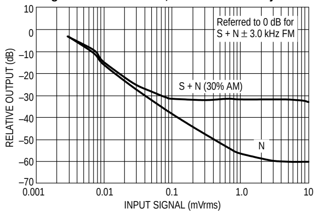
Figure 5. Overall Gain, Noise and AM Rejection
