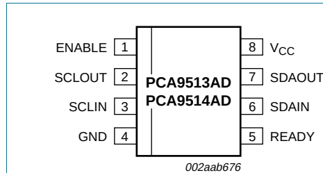
Fig 3. Pin configuration for SO8
