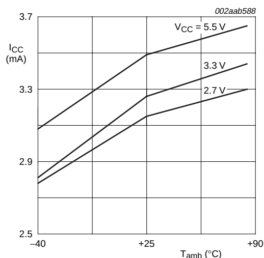
Fig 14. I_{\text{CC}} versus temperature
