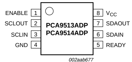
Fig 4. Pin configuration for TSSOP8 (MSOP8)
