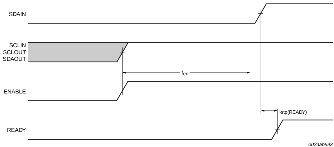
Fig 19. t_{stp(READY)} that can occur after t_{en}
