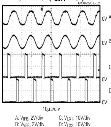
HIGH INPUT-VOLTAGE OPERATION ( V_{BATT} = 20V )
