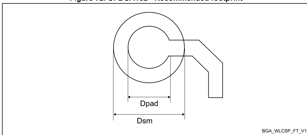
Figure 72. UFBGA132 - Recommended footprint
