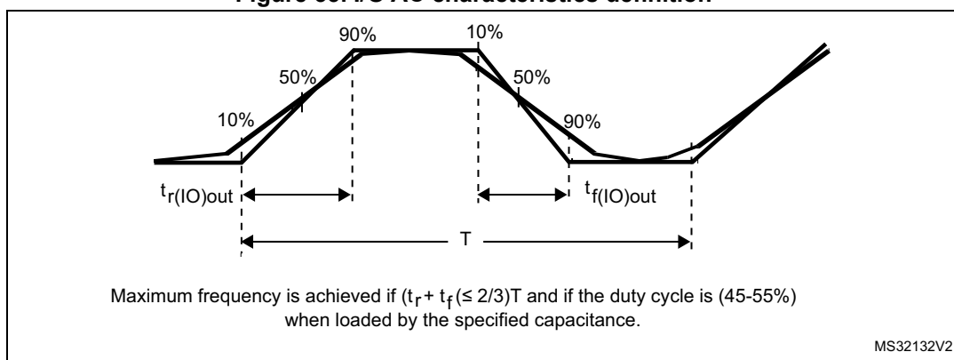
Figure 33. I/O AC characteristics definition (1)
