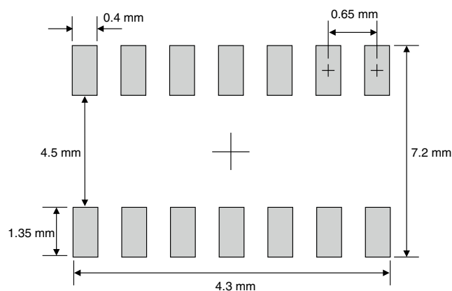
Fig. 5-4: Recommended pad size dimensions in mm
