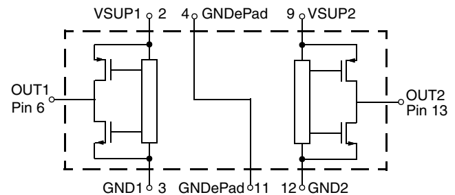
Fig. 4-3: Pin configuration
