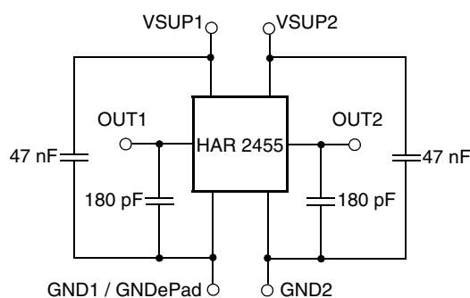
Fig. 5-2: Recommended application circuit (PWM output)
