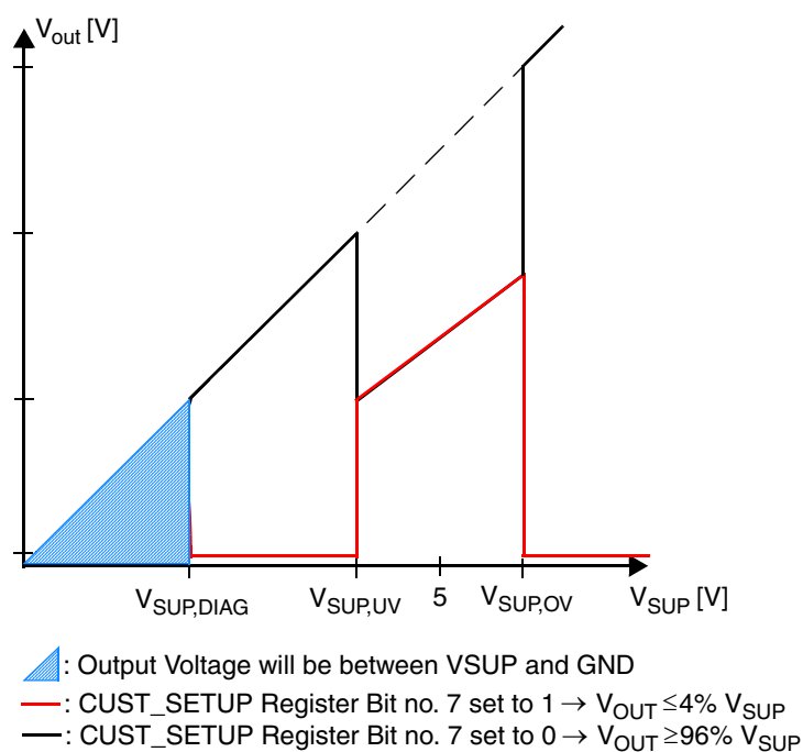
Fig. 4-5: Behavior of HAR 2425 for different V_{\text{SUP}}
