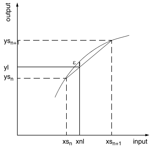
Fig. 3-8: Linearization - Detail
