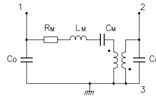
Equivalent LC Model
