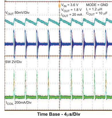
Figure 16. Typical Operation (PFM Mode)
