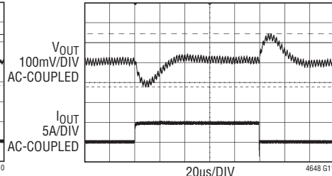
5V IN , 2.5V OUT Load Transient
