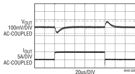
3.3V IN , 1V OUT Load Transient
