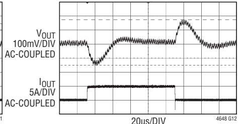
5V IN , 3.3V OUT Load Transient
