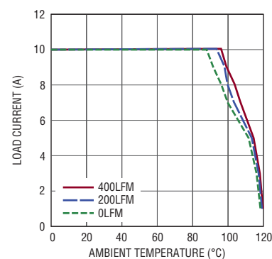
Current Derating, 5V to 1.5V OUT with No Heat Sink
