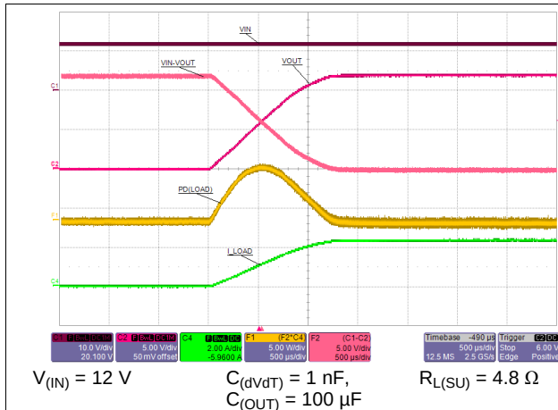
Figure 58. Typical Start-Up With Load
