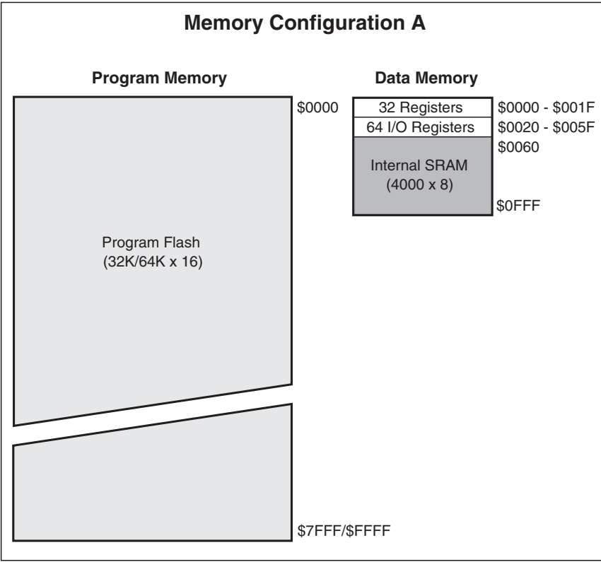
Figure 7. Memory Configurations
