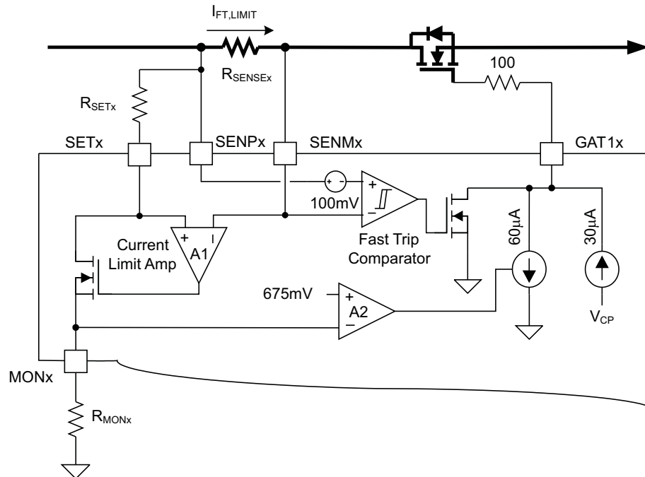
Figure 17. Overcurrent Protection Circuitry
