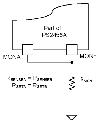
Figure 23. Fixed Fault Current Application
