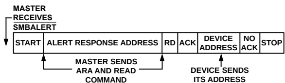
Figure 17. Use of SMBALERT
