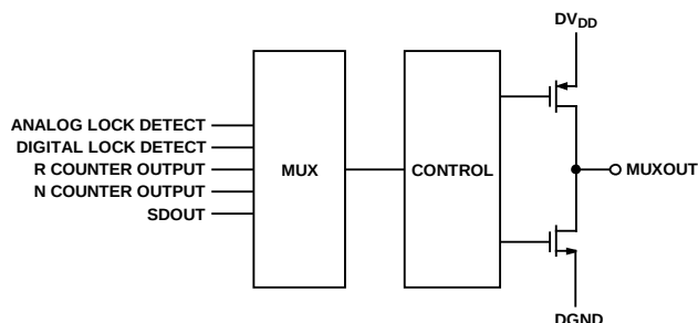
Figure 18. MUXOUT Circuit
