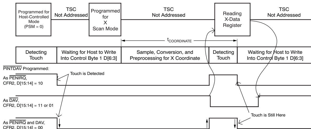
Figure 45. Example of a Single X Coordinate Touch Screen Scan (with Panel Stabilization Time) using TSMODE 3
