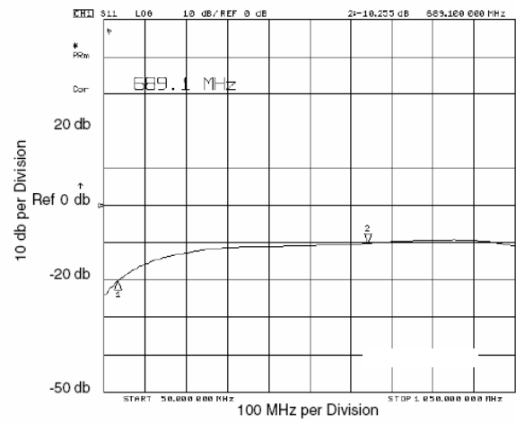
FIGURE 6 RETURN LOSS
