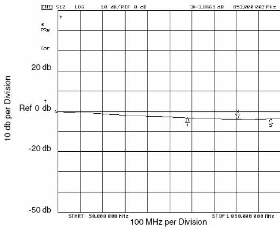
FIGURE 5 INSERTION LOSS
