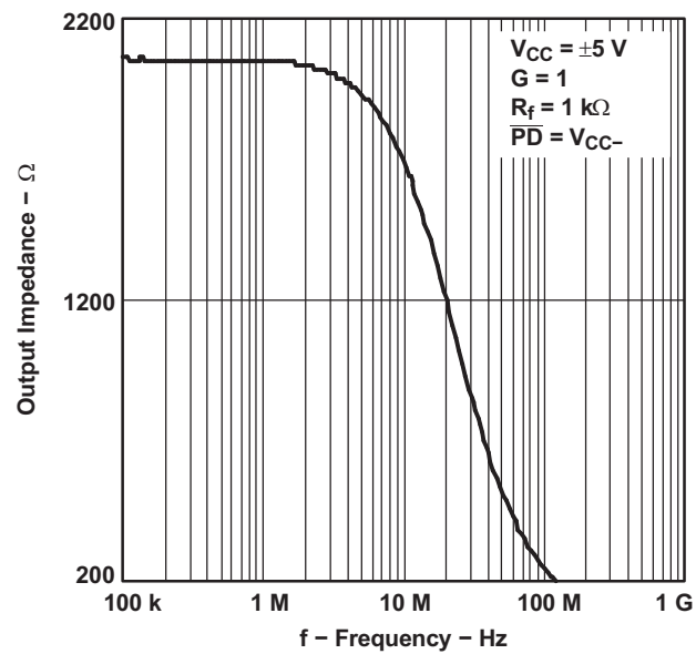
Figure 36. Output Impedance (in Power-Down) vs Frequency
