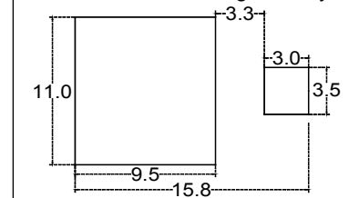
Recommended Mounting Pad Layout
