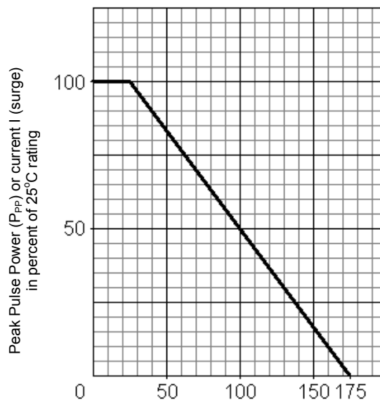
FIG. 4 Derating Curve
