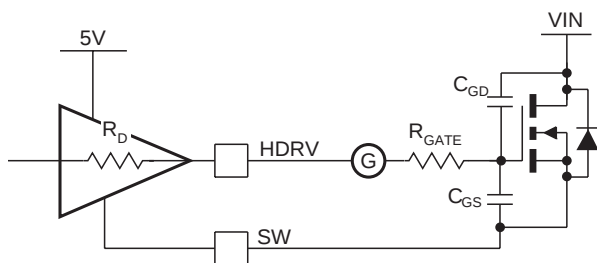
Figure 10. Drive Equivalent Circuit
