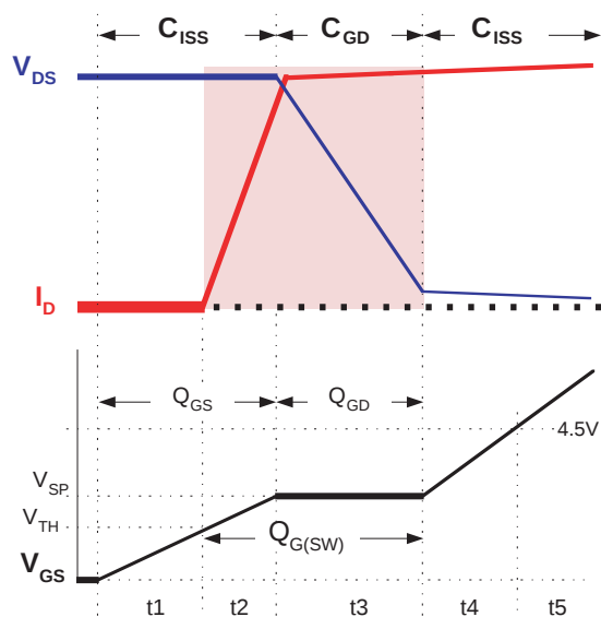
Figure 9. Switching Losses and Q_G
