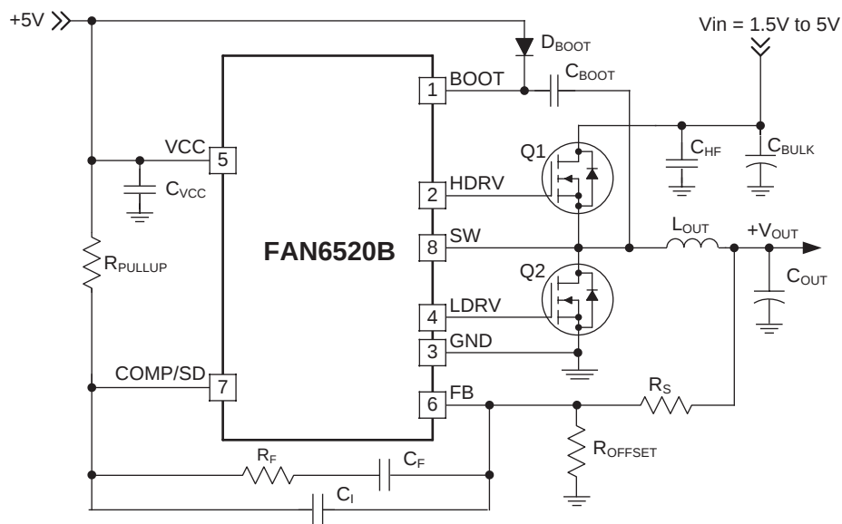
Figure 1. Typical Application
