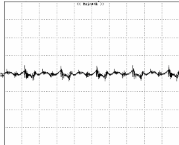
Figure 14: Output voltage ripple at nominal input voltage and rated load current ( I_o=20\text{A} ) ( 50\text{ mV/div} , 2\mu\text{s/div} ). Load capacitance: 1\mu\text{F} ceramic capacitor and 10\mu\text{F} tantalum capacitor. Bandwidth: 20\text{ MHz} . Scope measurements should be made using a BNC cable (length shorter than 20 inches). Position the load between 51 mm to 76 mm (2 inches to 3 inches) from the module.
