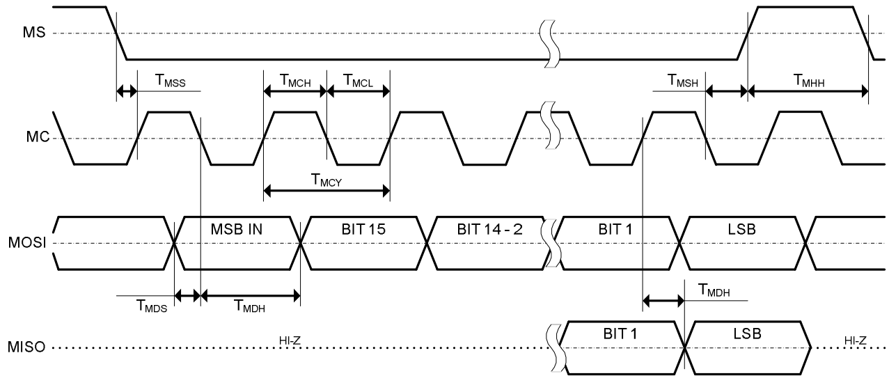
Figure 73. Control Interface Timing
