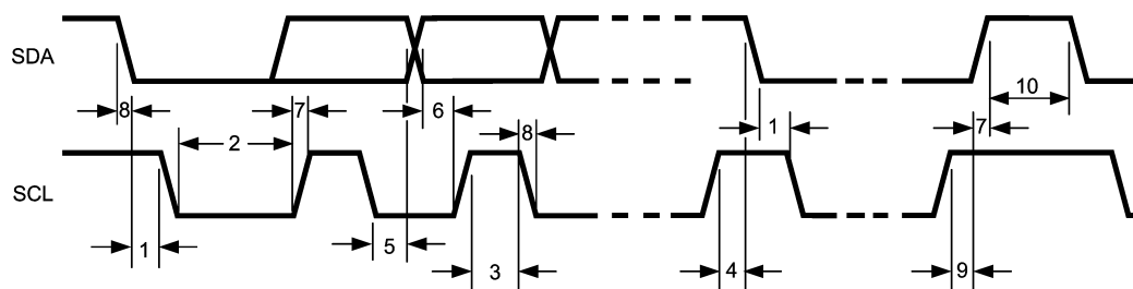
FIGURE 10. I 2 C Timing Diagram
