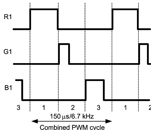
FIGURE 13. Normal Mode PWM Waveforms at Different Duty Settings
