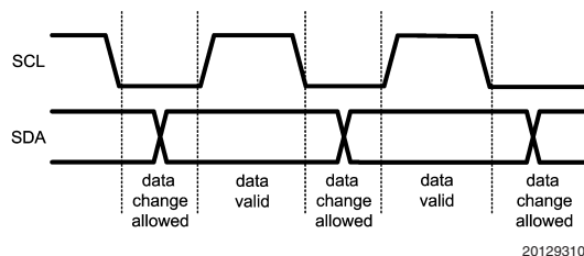
FIGURE 5. I 2 C Signals: Data Validity
